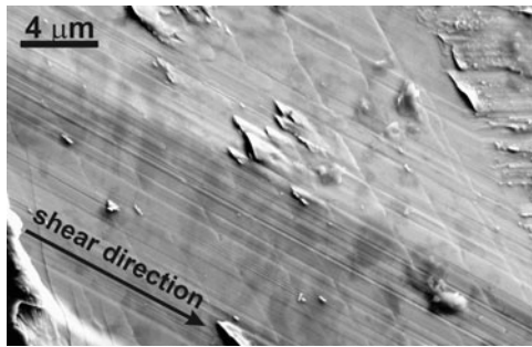
FIG. 3. Scanning electron microscopy image illustrating characteristic striations found on the glide surface exposed during shear. The spacing roughly corresponds to the glide distance during each cycle, demonstrating the intermittent nature of shear-band propagation.
