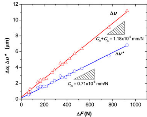
FIG. 5. Blue circles: Experimentally determined values of displacement burst magnitude \Delta u^* versus load-drop magnitude \Delta F , showing a linear trend with the slope reproducing the load-frame compliance C_m (blue fit). Red triangles: Corrected values of total displacement burst magnitude \Delta u taking into account the compliance of the entire system \kappa = (C_m + C_s) , with C_s being the compliance of a 5-mm-diameter sample. The compliance of the entire system, \kappa , corresponds to the slope of the red line.
